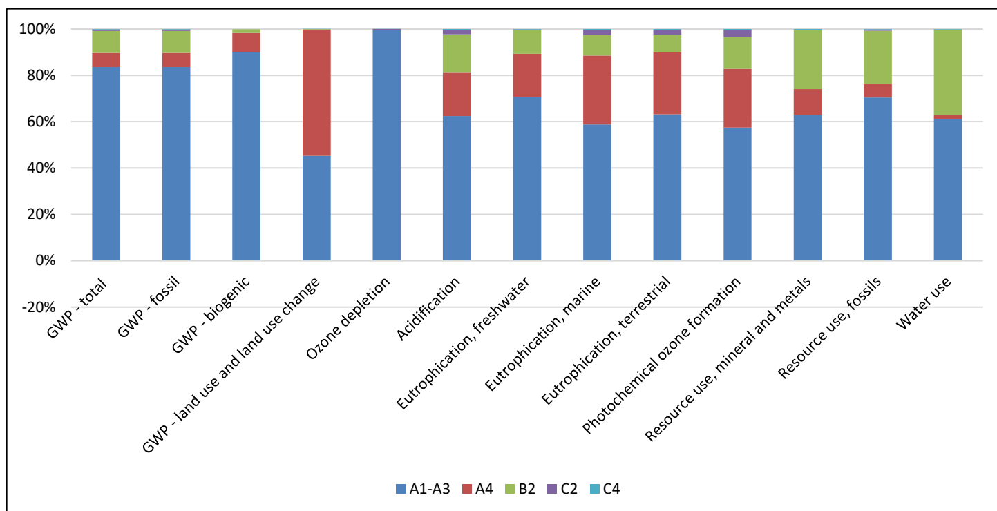
Figure 3 - Relative Contributions of Cradle to Gate Life Cycle Stages for Guardian UltraClear Flat Glass
