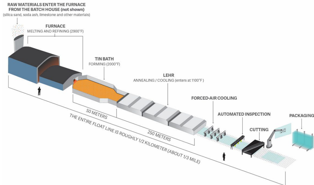
Figure 2 - Flat Glass Production
