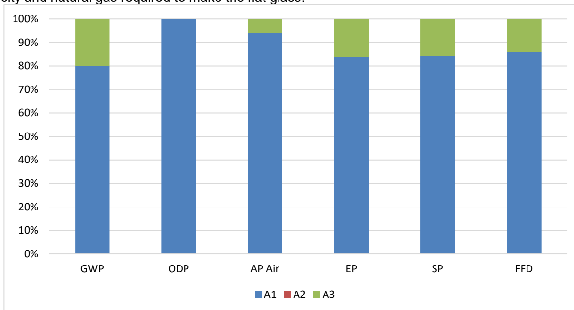
Figure 3 - Relative Contributions of Cradle to Gate Life Cycle Stages for Heat Treated Glass
