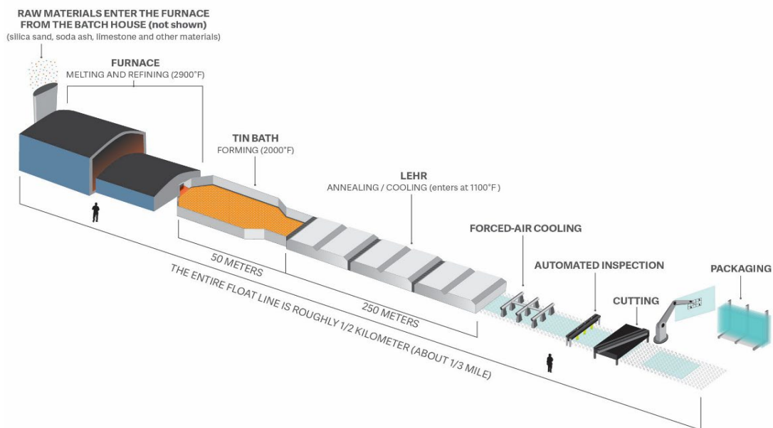
Figure 2 - Flat Glass Production Process
