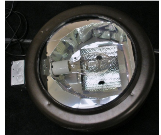
HID Fixture with Single Light Source and Reflectors
